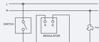
Fan Regulator with switch
