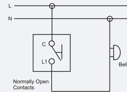
Bell Switch
