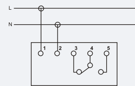
Programmable Timer - 24*7
