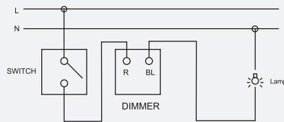
Dimmer with Switch
