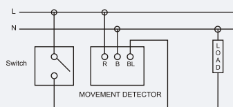
Movement Detector with bypass switch
