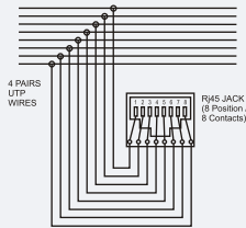
Computer Outlet - RJ45
