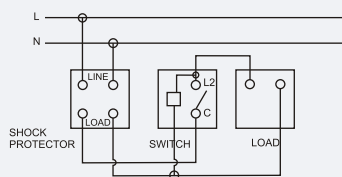
Shock Protector with Indicator Switch
