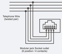
Telephone Outlet - RJ11
