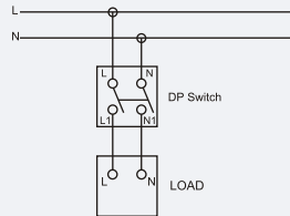
Double pole Switch
