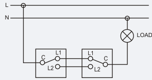
Two-Way Switch
