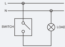
One-Way Switch
