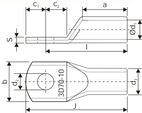
Copper Tubular Terminal Ends for solderless crimping to Copper Conductors
