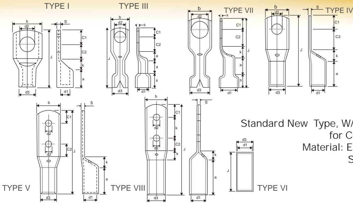
Copper Tubular Terminal Ends for solderless crimping to Copper Conductors
