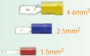
Male Disconnects
